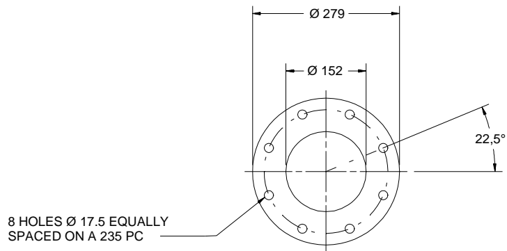
DETAIL OF EXHAUST OUTLET SCALE 1:5
